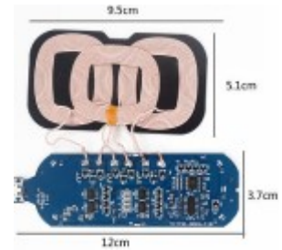
3-Coil Charger PCBA XH-PB-158 Size: PCBA + Coil
