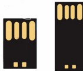
UDP Chip USB XH-USB-110 Size: 25 x 11 x 1.4mm
